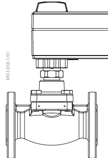
AME 10, AME 11 + VB 2 (DN 15-25)
